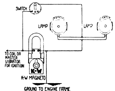
K-W MAGNETO ELECTRIC LIGHTING SYSTEM
